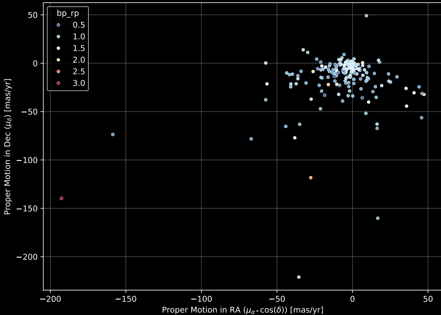
APOGEE DR17 Field: [197+31_MGA] Proper Motion Diagram (n= 202)
