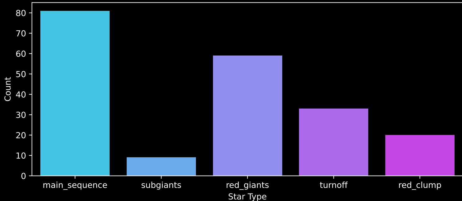
APOGEE DR17 Field: [197+31_MGA] Count plot of Star Type
