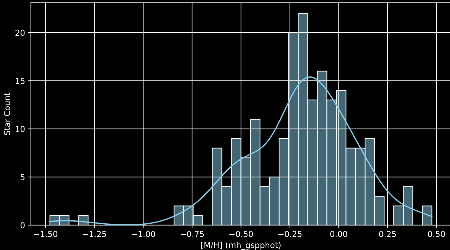
APOGEE DR17 Field: [197+31_MGA [M/H] (mh_gspphot) (n= 199)
